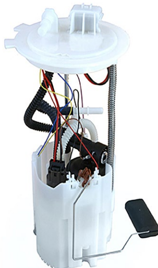
USEP21171M 2017-2022 Nissan Rouge Sport 2.0L; OE: 17040-6MA0A
